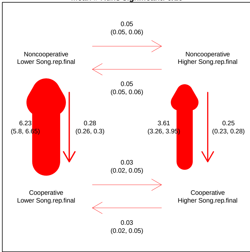
Thresholds \geq 1 - < 8.5 (23) Mean # Runs significant: 0/10
