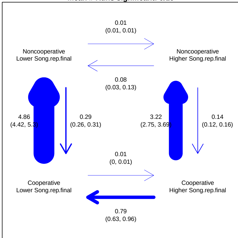
Thresholds \geq 34 - < 1450 (23) Mean # Runs significant: 0/10
