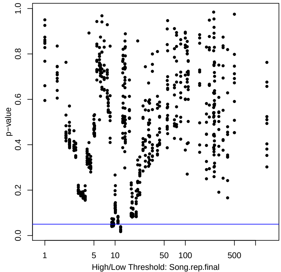
MeanCoopTie2Noncoop Song.rep.finalOriginal threshold range: 1 - 1450 (70)
