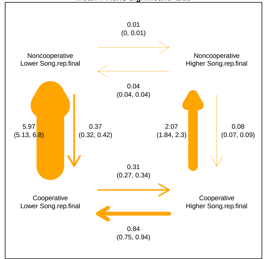
Thresholds \geq 8.5 - < 34 (24) Mean # Runs significant: 1/10
